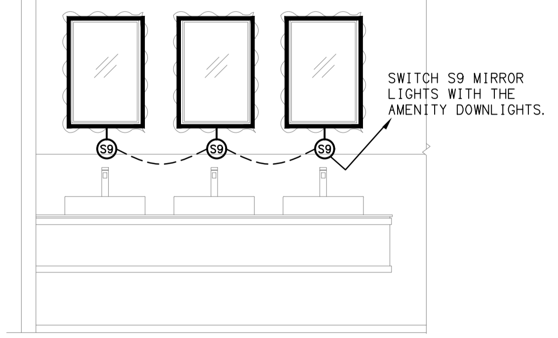
DETAIL A TYPICAL GAMING VANITY BENCH ELEVATION SCALE 1:25
